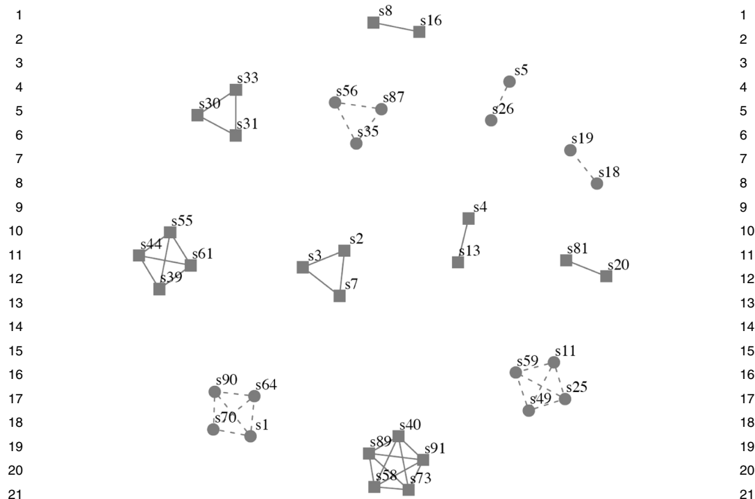
FIG. 1. Actual and recovered connectivities in the simulated data. The connectivities that were recovered by the clique loglinear models but were absent in the true connectivity graph are marked with dotted edges and round vertices. The connectivities marked with solid edges and square vertices give the true connectivity graph.
