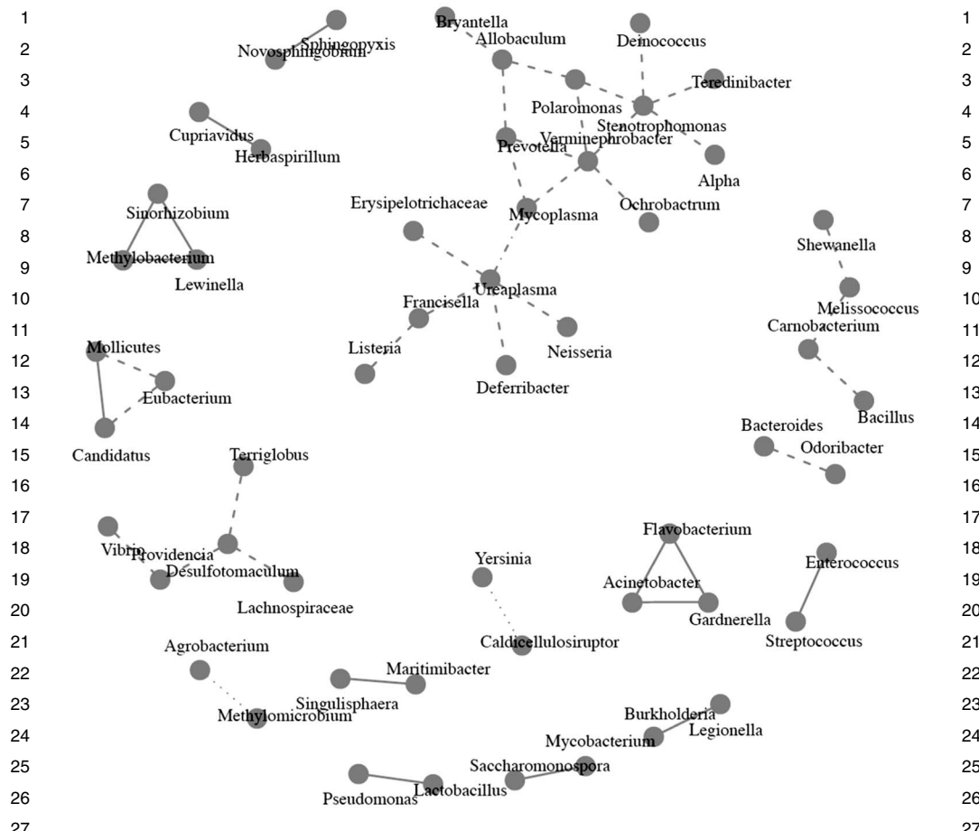
FIG. 4. Pairs of variables that have strictly positive posterior probabilities of belonging to an higher order term of a clique loglinear model in the genera data under the Occam's window BMA. Solid, dot dashed, dotted and dashed lines denote posterior probabilities that belong to the intervals (0.9, 1] , (0.5, 0.9] , (0.1, 0.5] and (0, 0.1] respectively.
