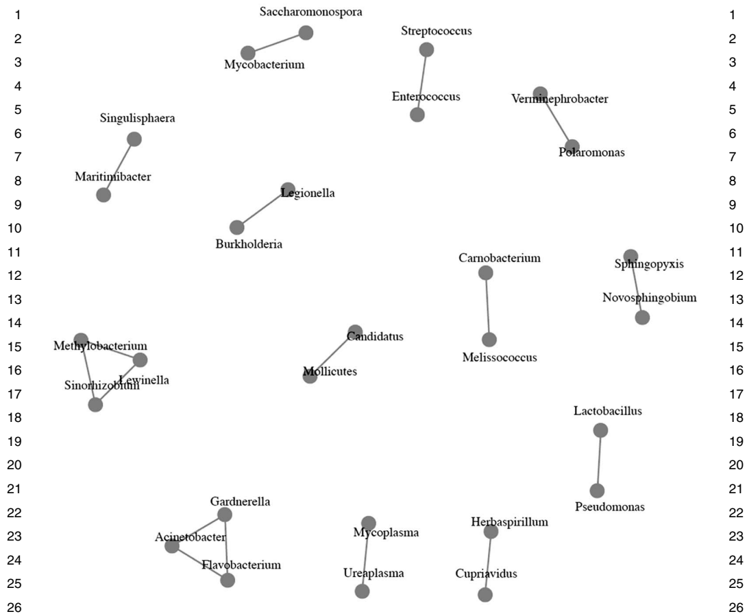
FIG. 3. The best clique loglinear model identified for the genera data.
